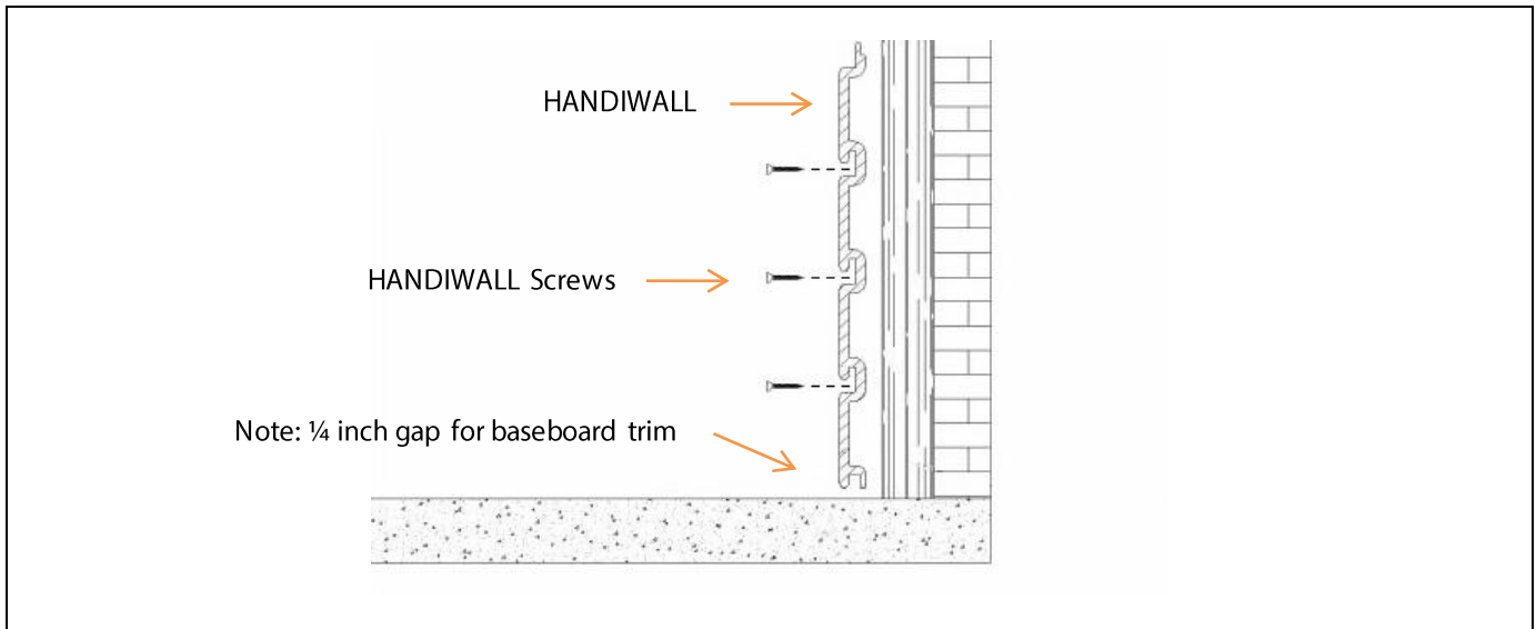
Figure 2. HANDIWALL Installation
